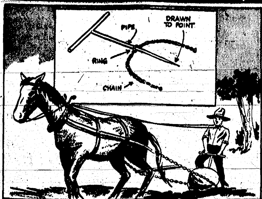
Device for removing stones from field employs chain and T-pipe. Chain is passed around stone with pipe extending through ring in chain into ground under stone. The pull of the horse and prying of the man dislodge stone.
